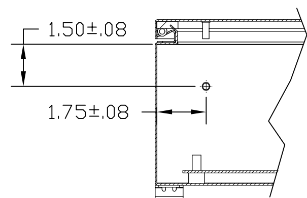
SECTION Z-Z SHOWING BOX GROUND STUD LOCATION
